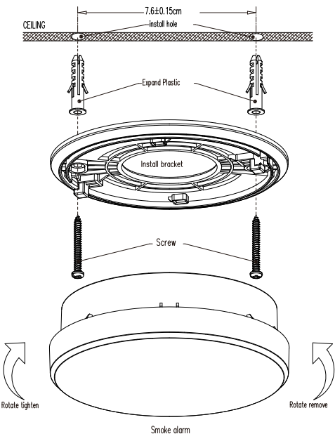
DIAGRAM 4 Installation Sketch Map
