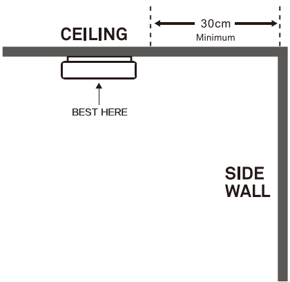
DIAGRAM 2 CEILING PLACEMENT
